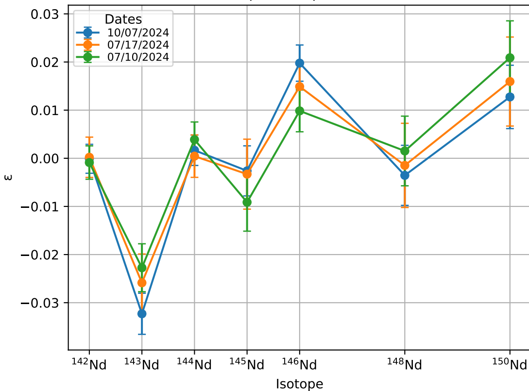
\epsilon Trends vs. Isotopic Composition for Each Date
