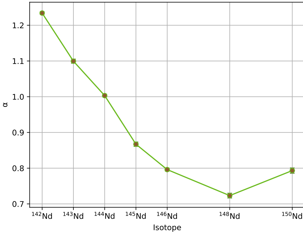
Combined Data \alpha Trends as a Function of Isotopic Composition
